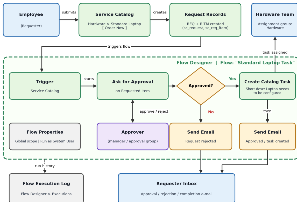
Figure 1: Architecture and data flow of the automated Standard Laptop ordering process in ServiceNow
